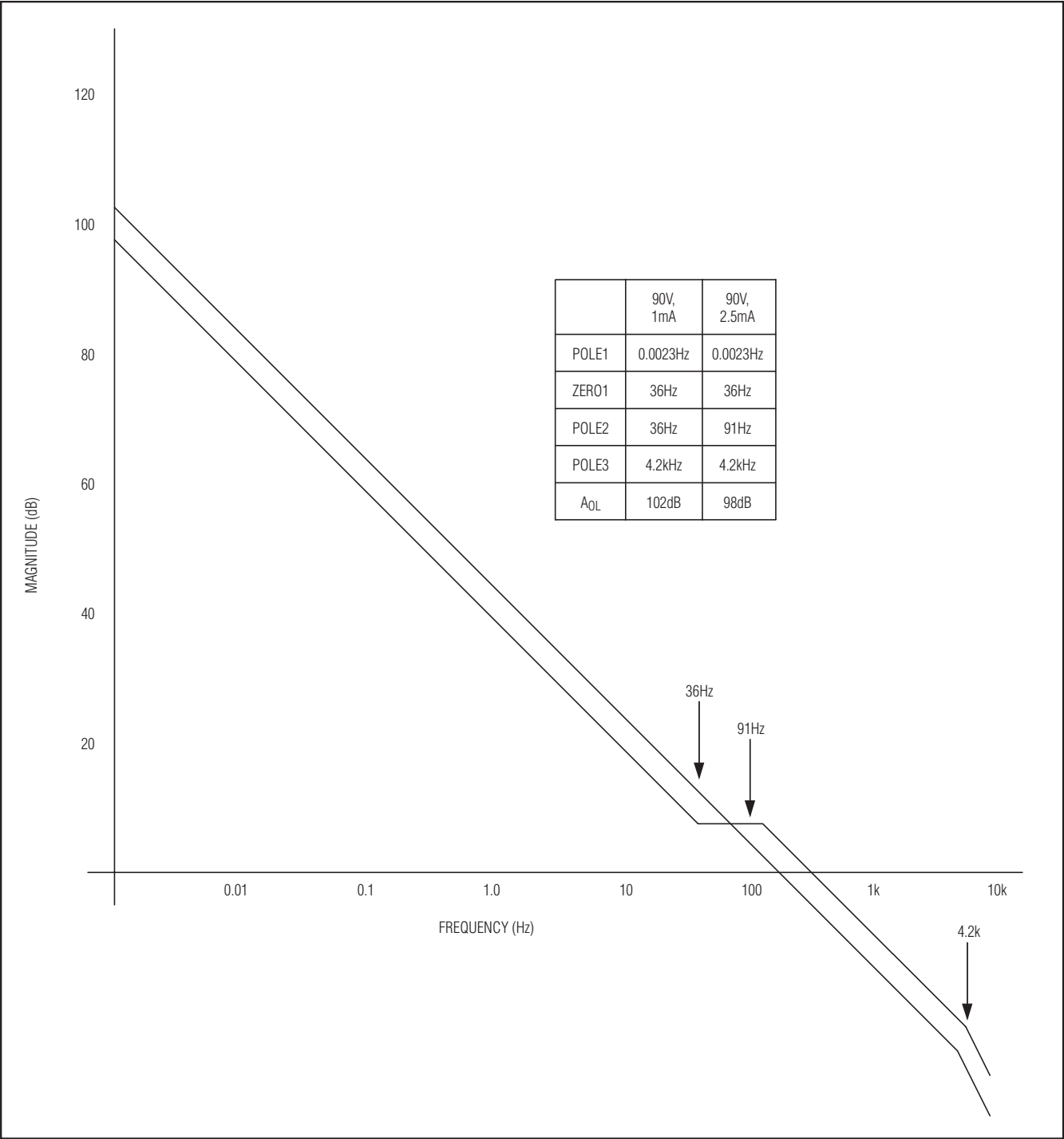
Figure 6. Loop Response
