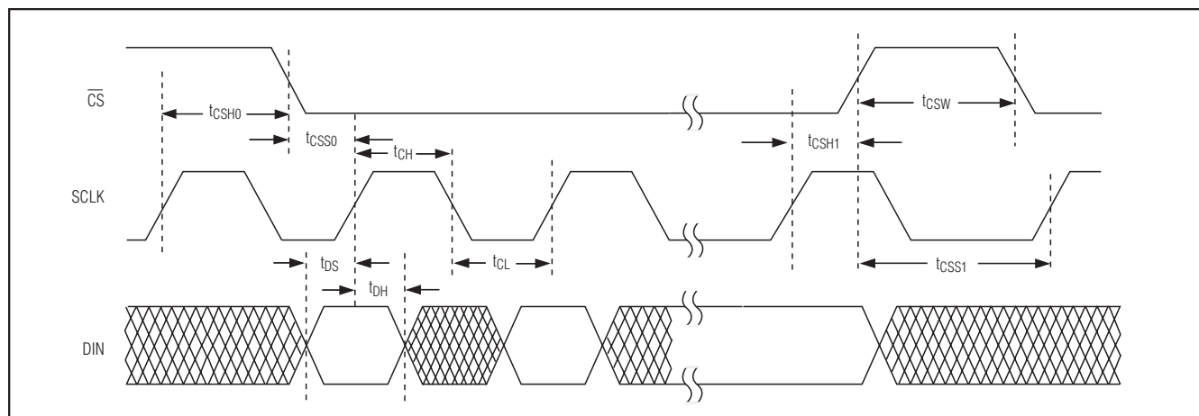
Figure 5. Detailed Serial Interface Timing Diagram
