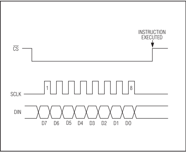
Figure 4. Serial Interface Timing Diagram
